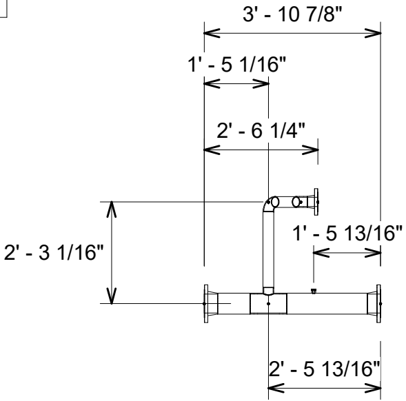
3 Pipe Elevation View
