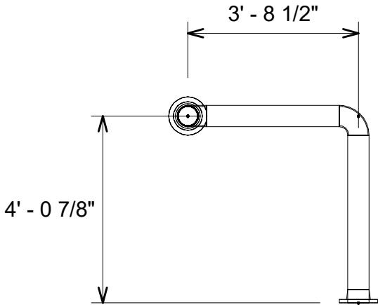
3 Pipe Elevation View
