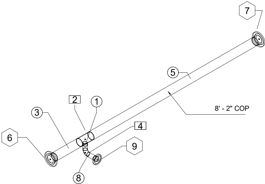
1 Pipe Iso View
