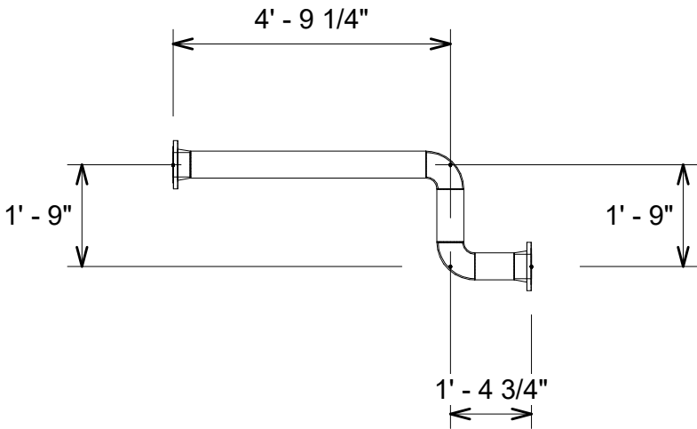
3 Pipe Elevation View
