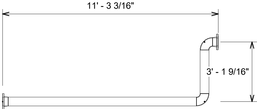
3 Pipe Elevation View
