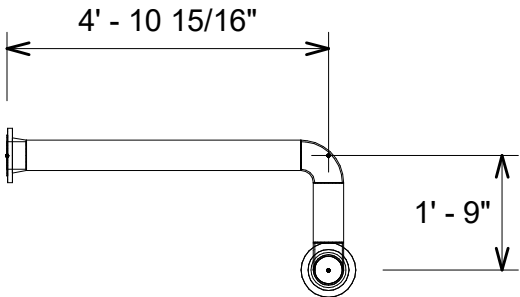
3 Pipe Elevation View
