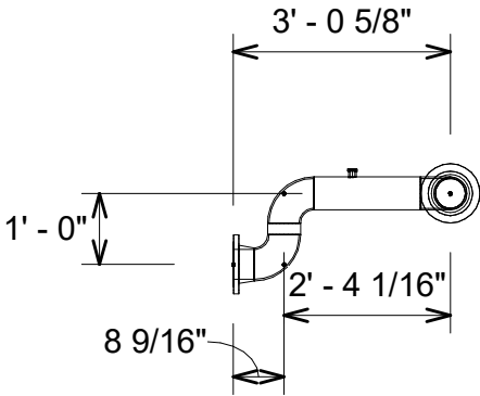
3 Pipe Elevation View
