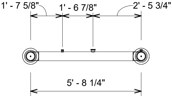
3 Pipe Elevation View
