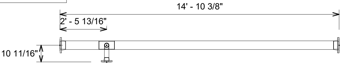
2 Pipe Plan View
