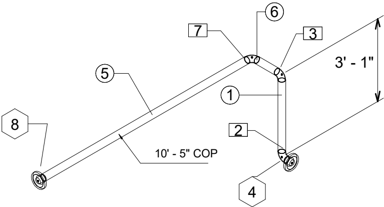
1 Pipe Iso View
