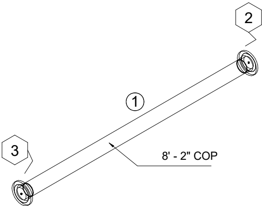
1 Pipe Iso View
