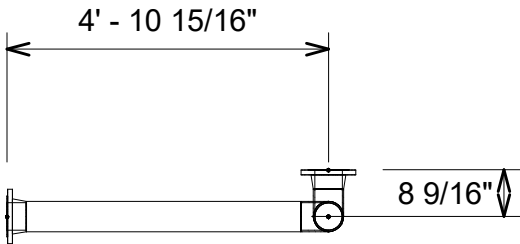
2 Pipe Plan View
