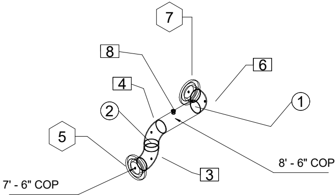
1 Pipe Iso View
