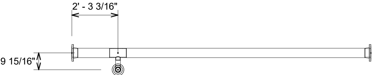
3 Pipe Elevation View
