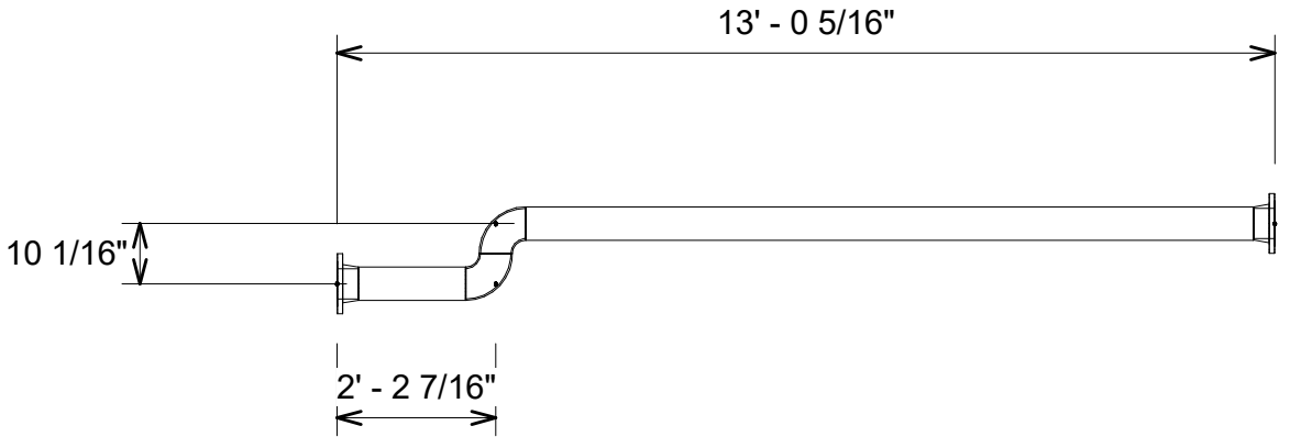
3 Pipe Elevation View
