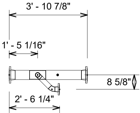
2 Pipe Plan View
