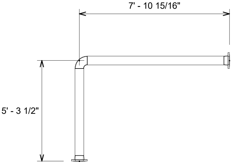
3 Pipe Elevation View
