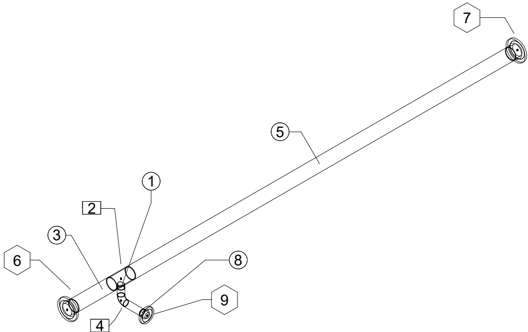
1 Pipe Iso View
