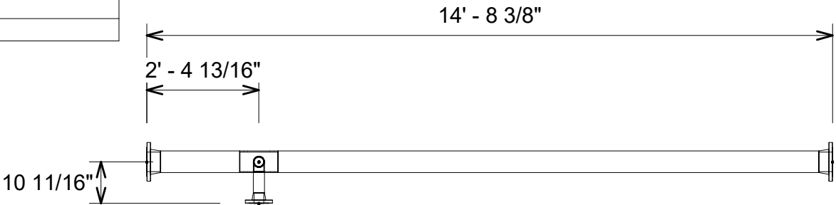
2 Pipe Plan View
