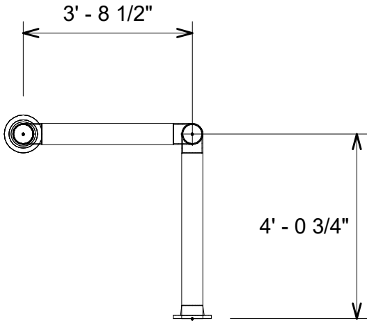
3 Pipe Elevation View
