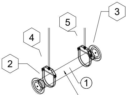
1 Pipe Iso View
