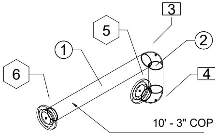
1 Pipe Iso View
