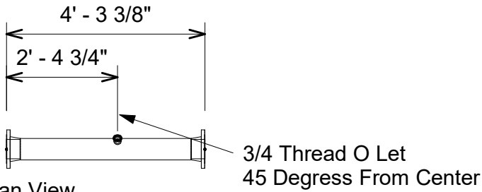
2 Pipe Plan View
