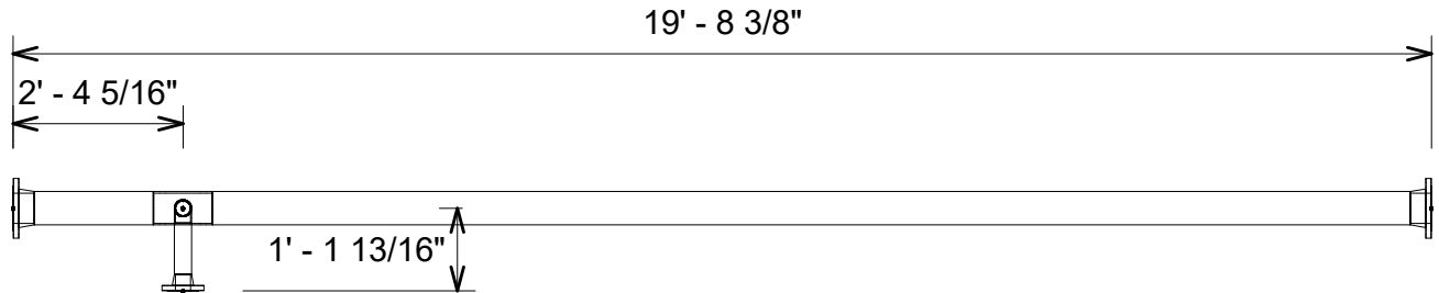
2 Pipe Plan View
