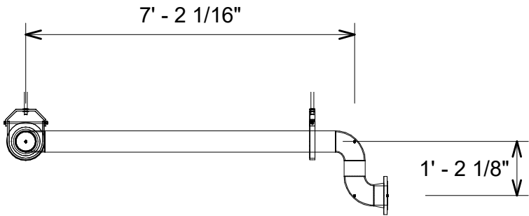
3 Pipe Elevation View
