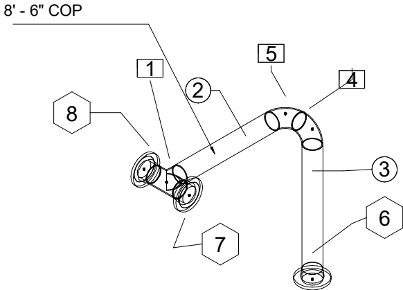
1 Pipe Iso View
