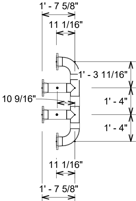
2 Pipe Plan View
