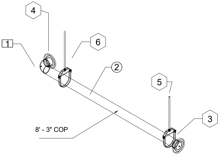
1 Pipe Iso View
