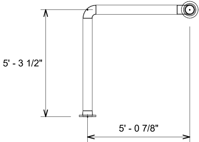
3 Pipe Elevation View
