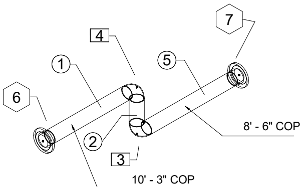
1 Pipe Iso View
