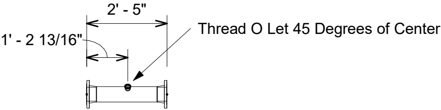
2 Pipe Plan View
