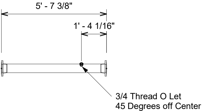
2 Pipe Plan View
