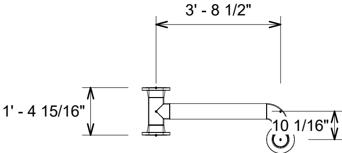
2 Pipe Plan View
