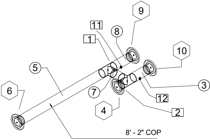
1 Pipe Iso View
