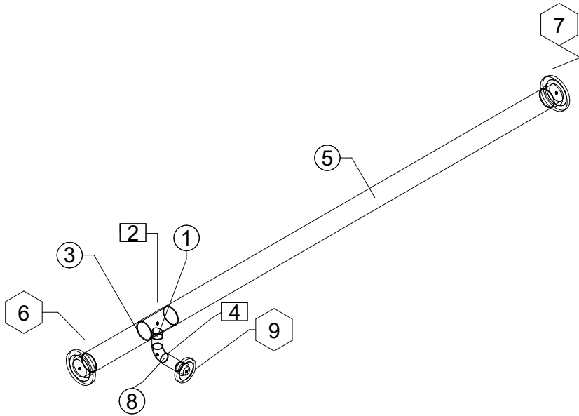
1 Pipe Iso View
