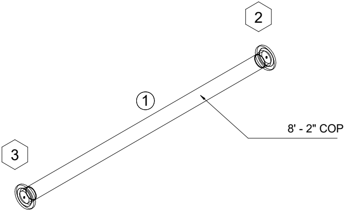
1 Pipe Iso View
