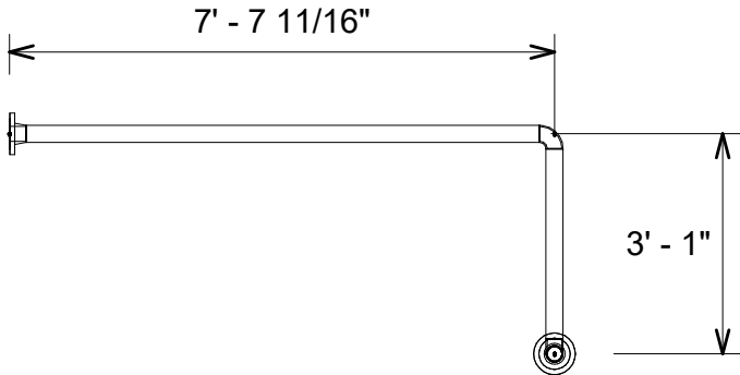
3 Pipe Elevation View
