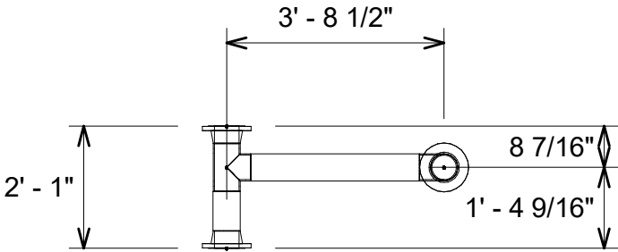
2 Pipe Plan View
