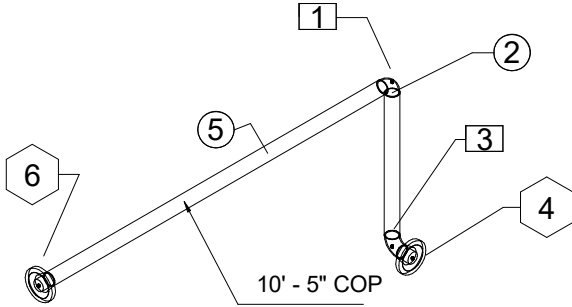
1 Pipe Iso View
