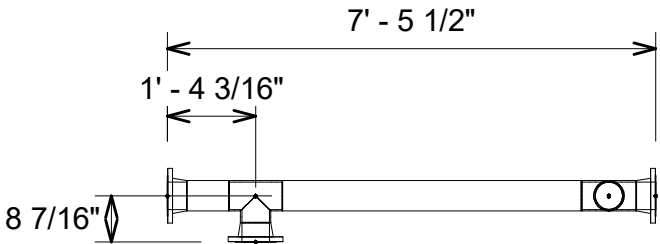
2 Pipe Plan View
