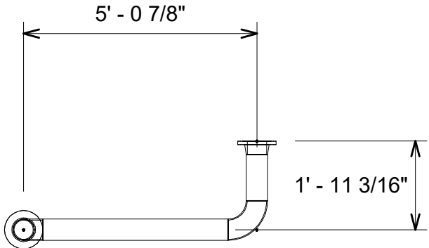
2 Pipe Plan View
