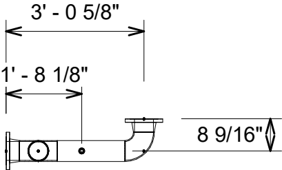
2 Pipe Plan View
